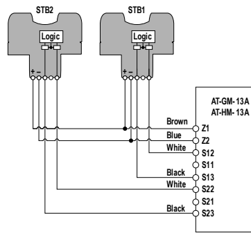
Figure 6. Hookup to two STB touch buttons with PNP (sourcing) outputs
