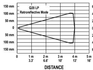
Beam Pattern
