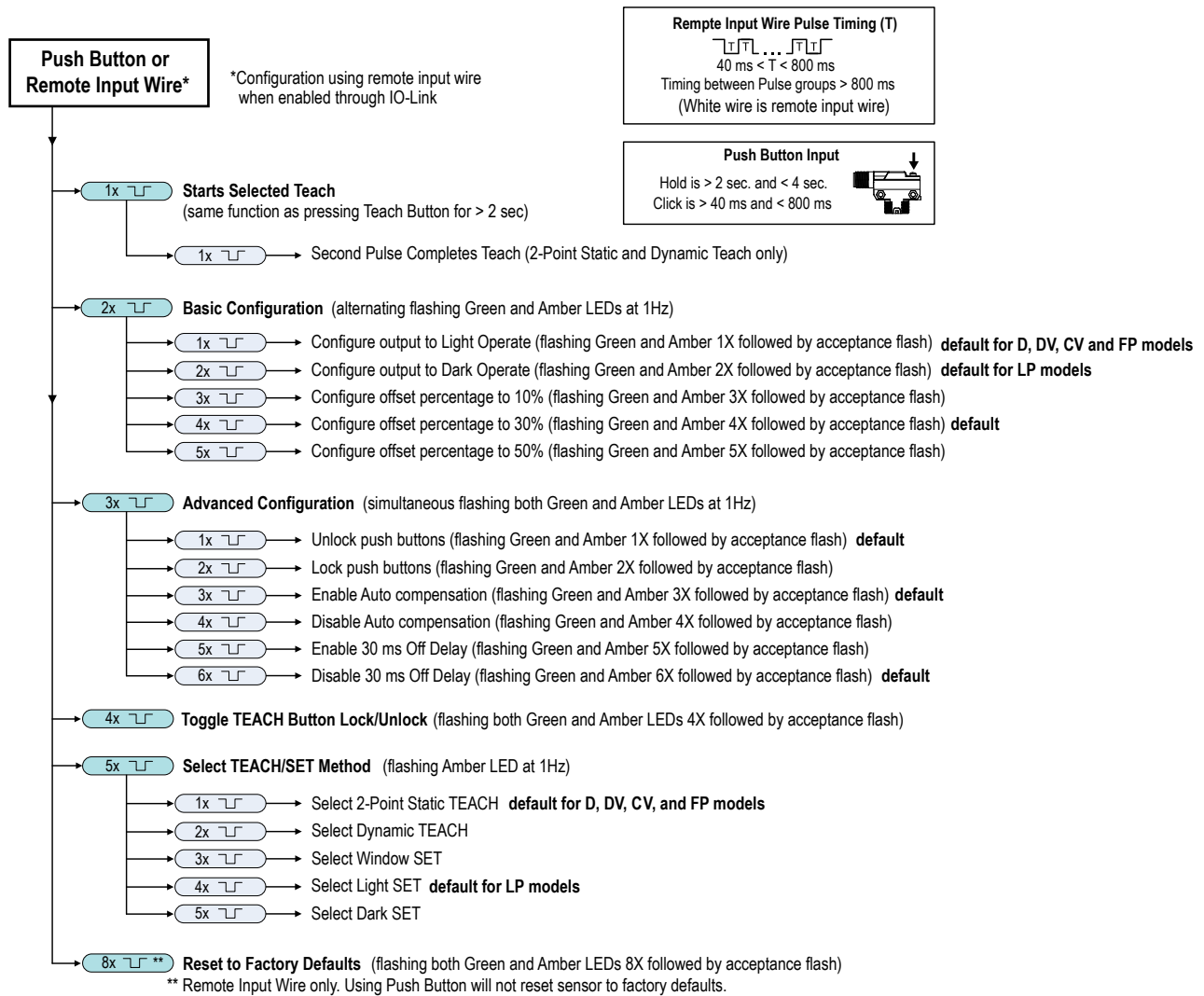
Figure 7. Input Flowchart
