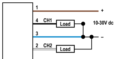
Figure 4. Channel 1 = PNP Output, Channel 2 = PNP Output
