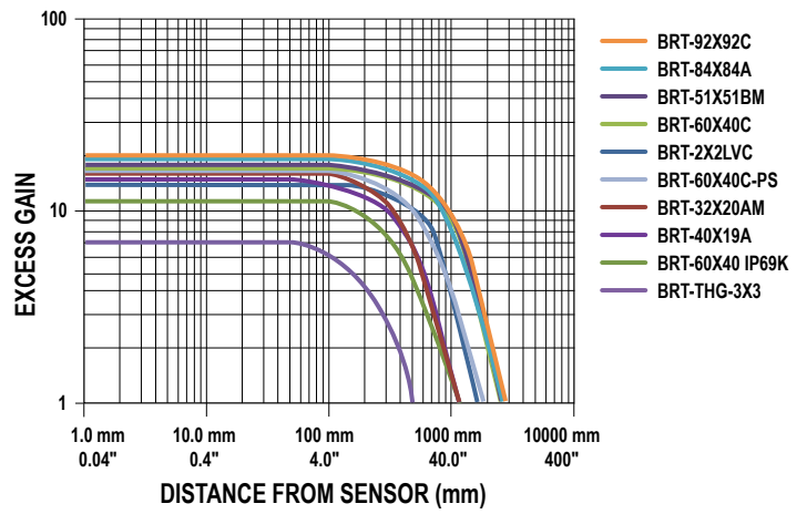
Excess Gain
