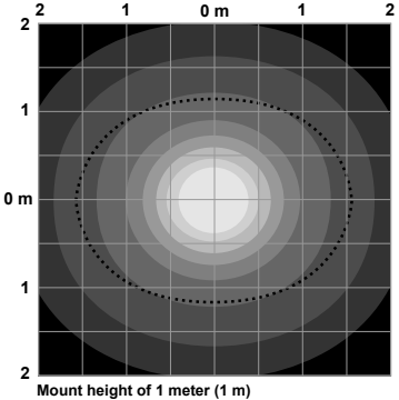
Isolux Pattern
