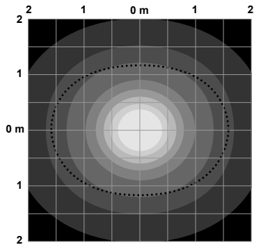
Isolux Pattern
